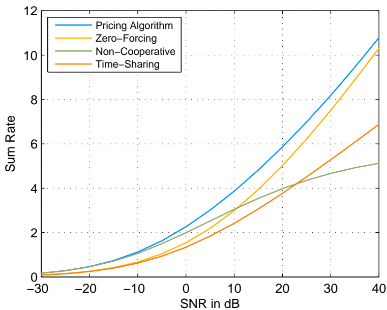
Fig. 5. Illustration of the sum rate versus SNR for different algorithms
