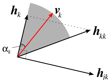
Fig. 6. Illustration of the optimal beamformer v_k in a two user network. The shaded area denotes the convex cone spanned by the channel matched filter and the zero-forcing beamformer. The boundary of this region corresponds to those beams that meet the power constraint.
