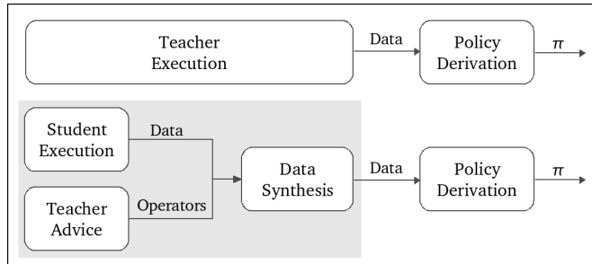
Fig. 1. Generating demonstration data. Typical approaches provide demonstration data from teacher executions (top). Our approach introduces a novel technique for generating data based upon learner executions and teacher advice (bottom, shaded box).
