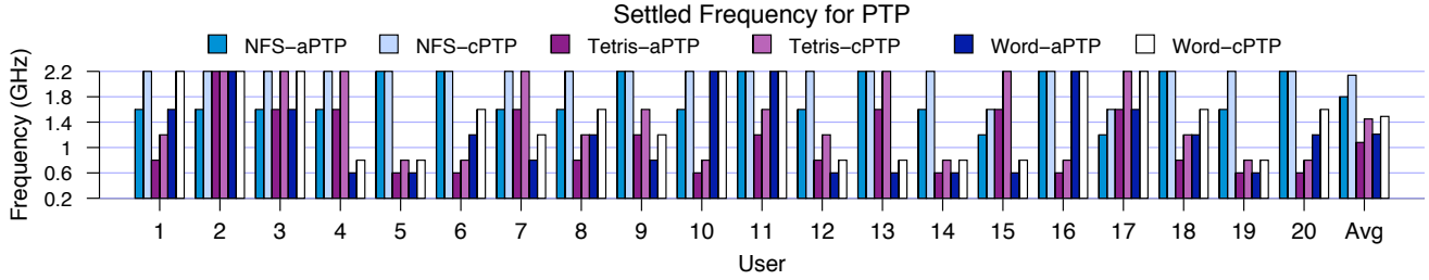
Figure 7. Frequency that a PTP and c PTP settle on for the Need for Speed, Tetris, and Word applications.
